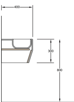
DfE3 Thermo Profile Thermoformed trough with deck mounted taps. A choice of underframe or brackets.
