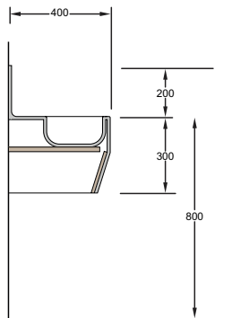
DfE2 Thermo Profile Thermoformed trough with deck mounted taps. A choice of underframe or brackets.
