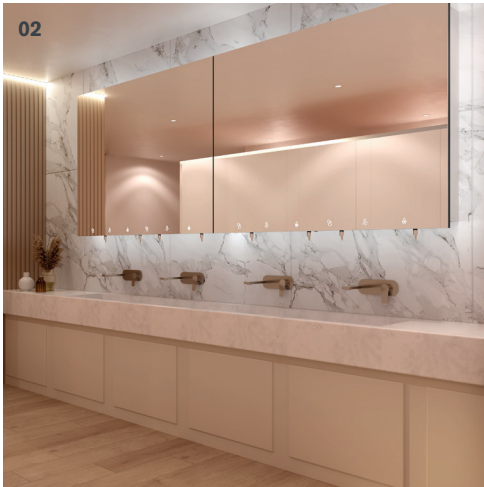
02 WT2 profile Solid Surface thermoformed sloped washtrough in Roman Marble and Suede HPL underpanels with Hartley wall mounted mixer taps in brushed nickel. Infinite HPL cubicles in Porcelain with 1300mm Mirror Box Units with liquid soap dispensers, hand sanitiser dispensers and automatic hand dryers.
