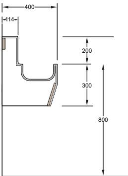
DfE1 Thermo Profile Thermoformed trough with wall mounted taps. A choice of underframe or brackets.
